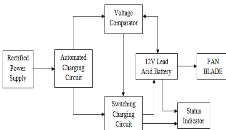
Figure 1: Block Diagram of the Rechargeable Electric Fan
