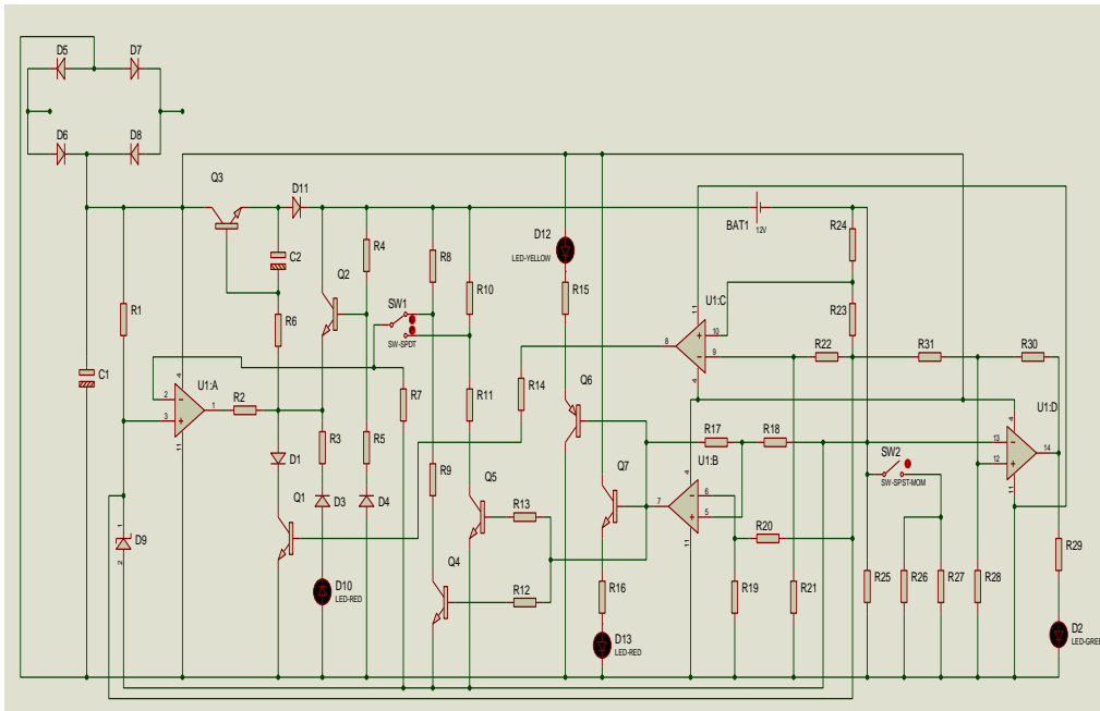
Figure 2: Automated Charging Circuit Diagram
