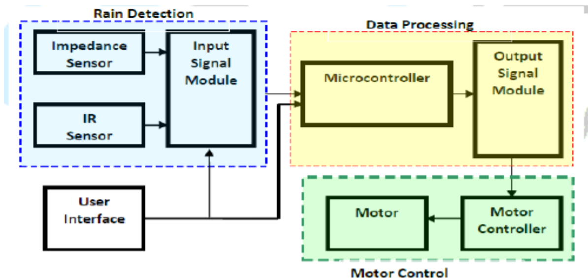
Fig. 1: Architecture diagram
