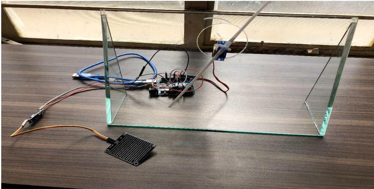
Fig. 4: Hardware Model
