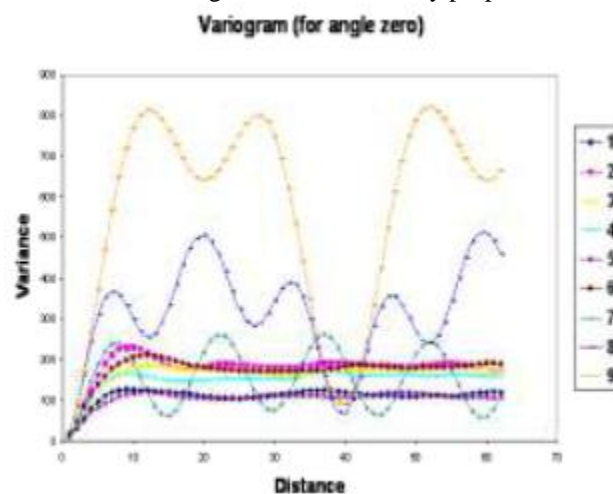
Figure 4c: Variogram of image in figure 4b
