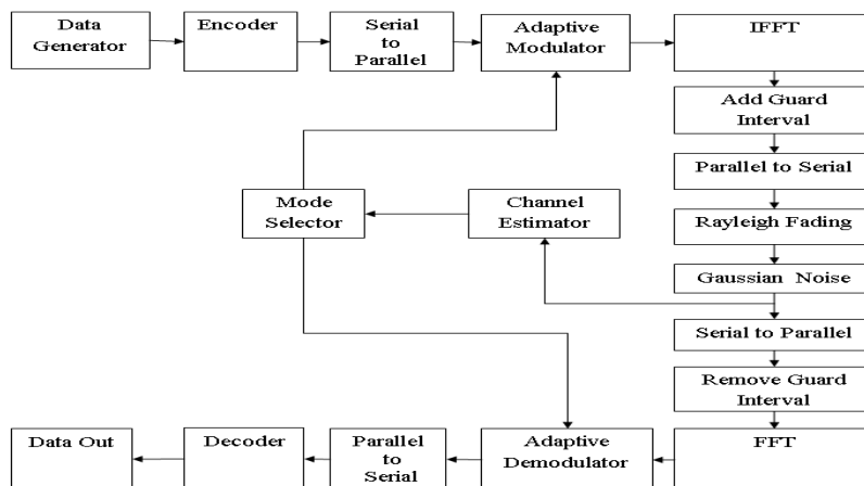
Figure 1. Adaptive OFDM system
