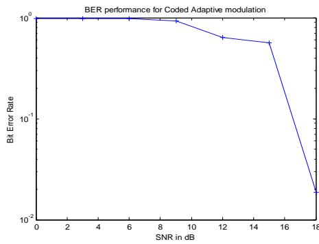
Figure 2. BER Performance of Coded AOFDM With BPSK, QPSK, QAM
