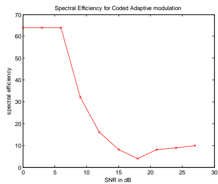
Figure 5. Spectral efficiency of Coded AOFDM with BPSK, QPSK, QAM
