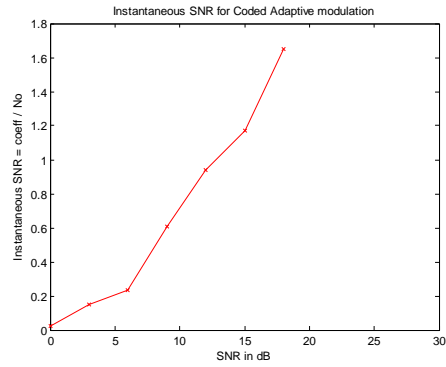
Figure 3. Instantaneous SNR of Coded AOFDM with BPSK, QPSK, QAM
