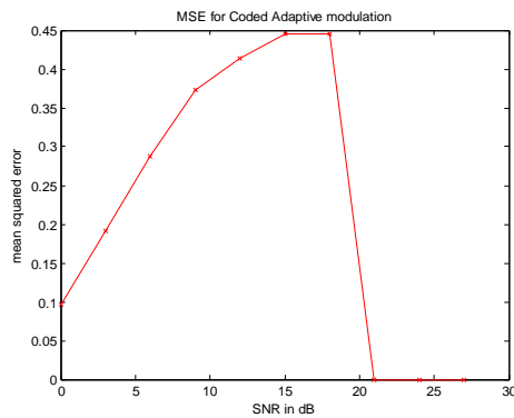
Figure 4. Mean Square Error of Coded AOFDM with BPSK, QPSK, QAM
