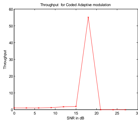
Figure 6. Throughput of Coded AOFDM with BPSK, QPSK, QAM
