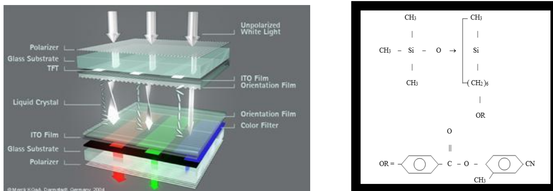
Fig. (1). Electro-optic cell.
