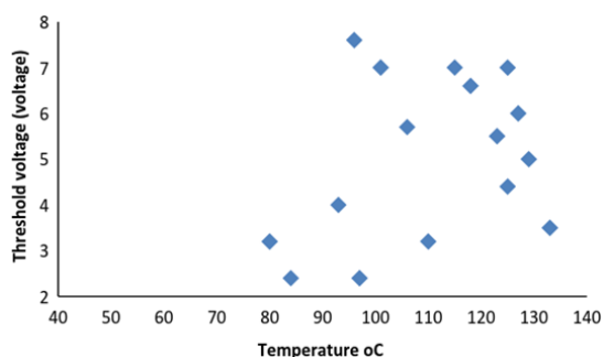
Fig. (7).Plots of the measured threshold voltages a function of temperature
