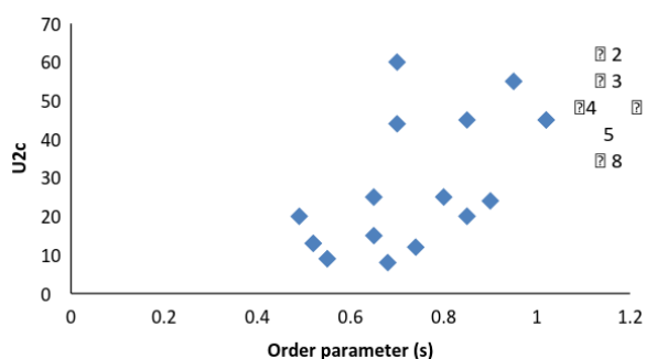
Fig. (8). A plots showing square of the threshold voltages against the order parameter S
