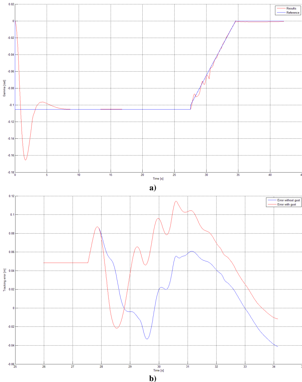
Fig. 3 Indirect flight path following with gust: a) Desired and controlled flight path angle, b) tracking error comparison
