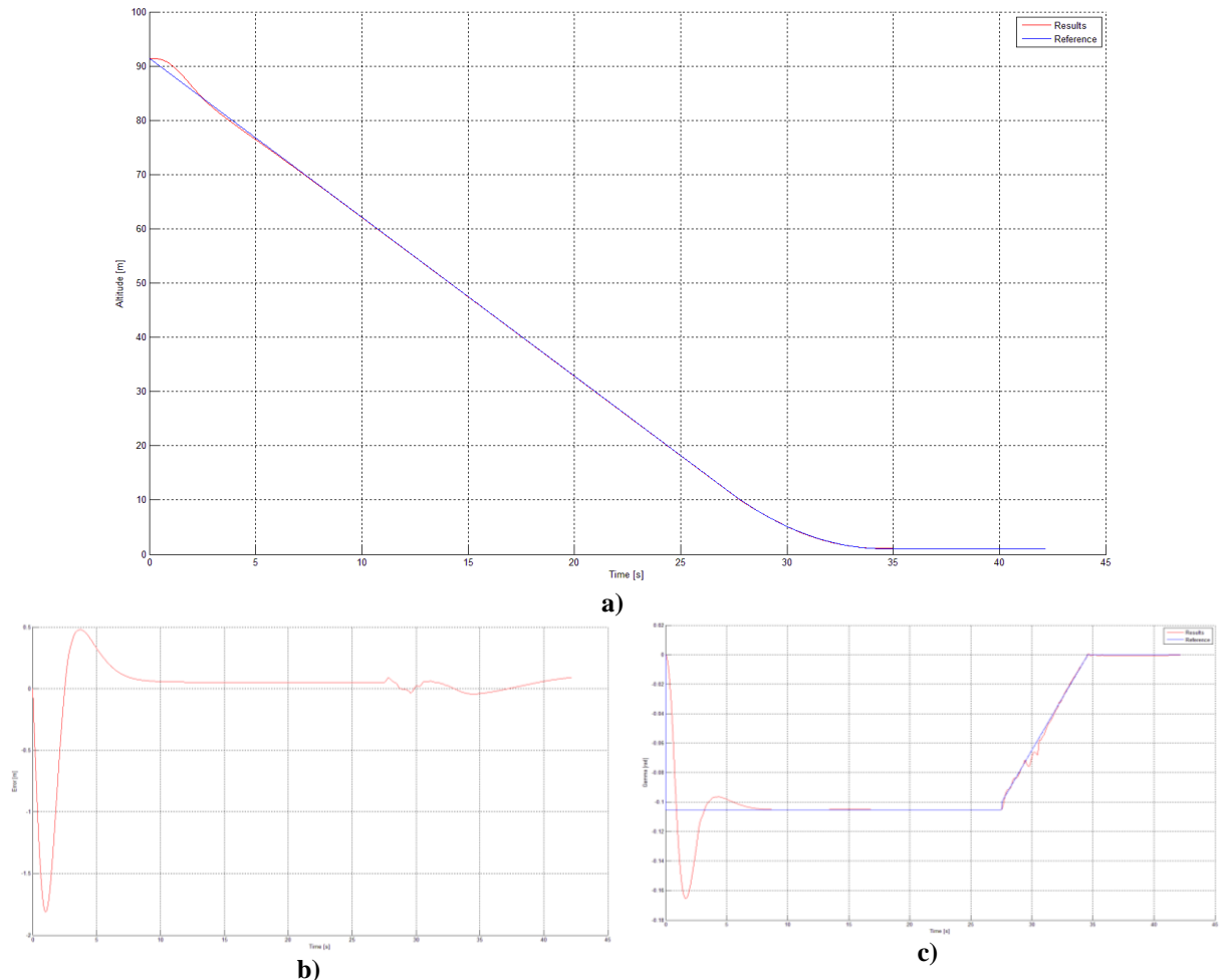
Fig. 2 Indirect flight path following:
