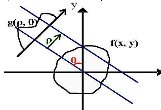
Figure 1 - Illustration of Radon transform.
