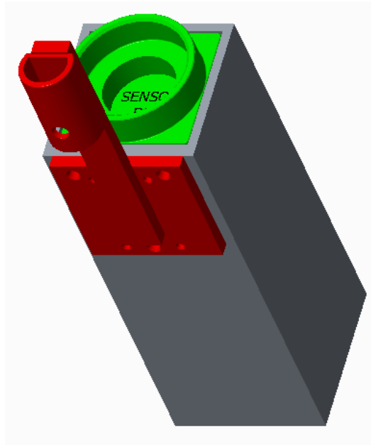
Figure 3 - Laser and Camera Mount
