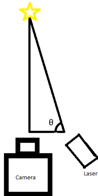
Figure 4 - Laser offset Diagram
