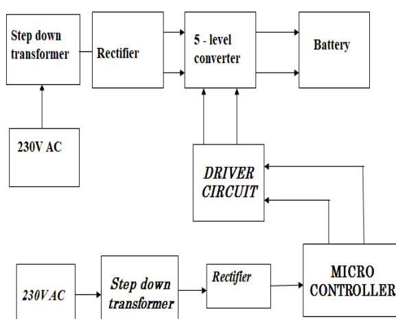
Fig.6.Block diagram of hardware experimental setup of 5 level converter
