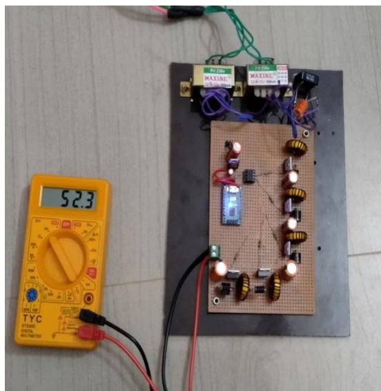
Fig 7: Hardware Setup
