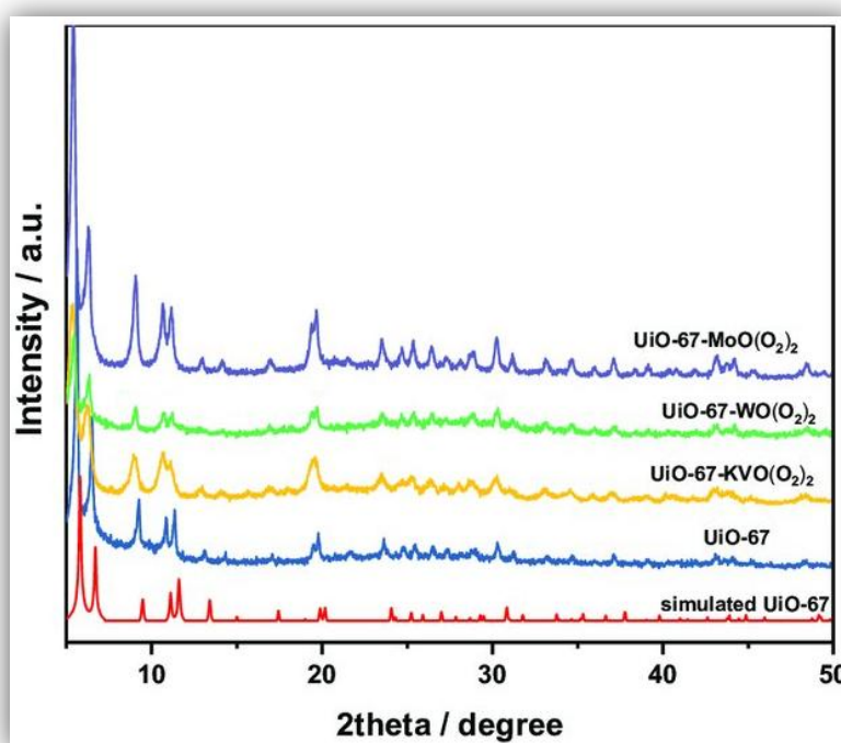
Fig 9.XRD patterns of the simulated UiO-67 and the synthesized UiO-67, UiO-67-MoO(O 2 ) 2 , UiO-67-WO(O 2 ) 2 , and UiO-67-KVO(O 2 ) 2 . [29]
