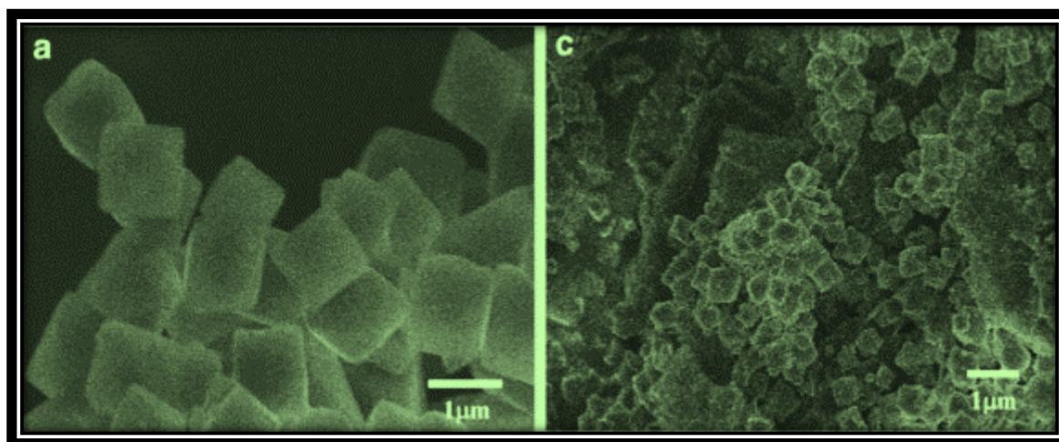
Fig8. SEM images of UiO-67 samples obtained doxorubicin: (a)UiO-67, (c) UiO-67- doxorubicin.
