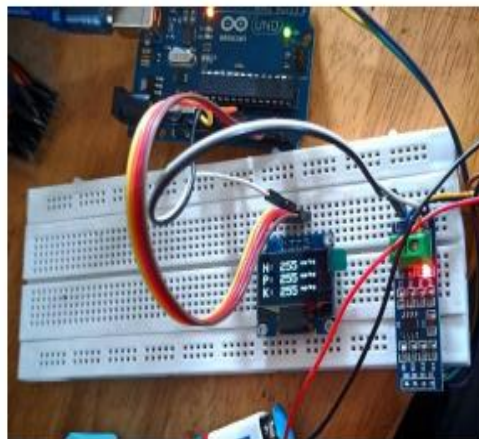
Fig 3(a).Hardware connection of Soil Moisture sensor
