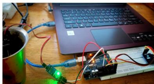
Fig 3(b).Hardware connection of soil NPK Sensor
