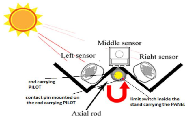
Fig- 3 Sensing mechanism mounted on the PILOT.
