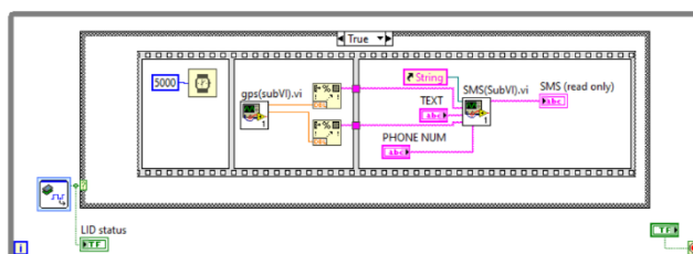
Figure.1a LabVIEW interfaced block diagram
