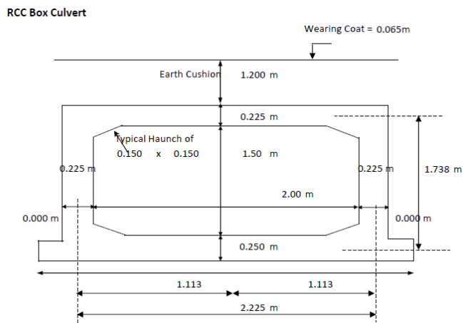
Figure No. 3 Box Culvert with Cushion thickness 1.200m
