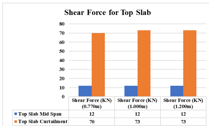
Graph No. 4 Shear force for Top Slab
