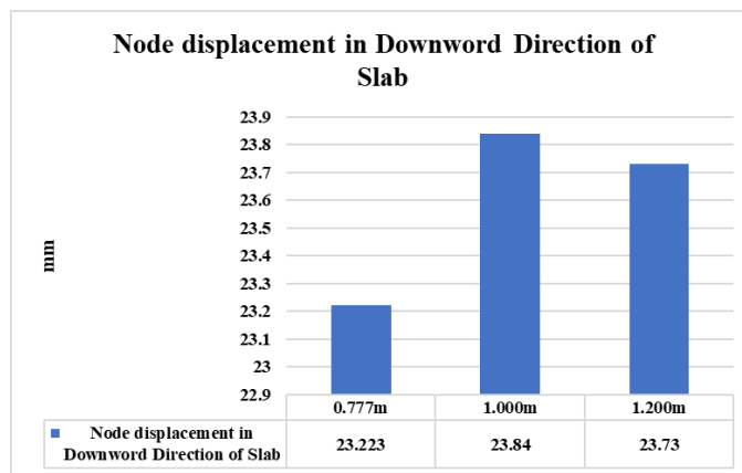
Graph 7 Node Displacement in Downwards Directions of top slab
