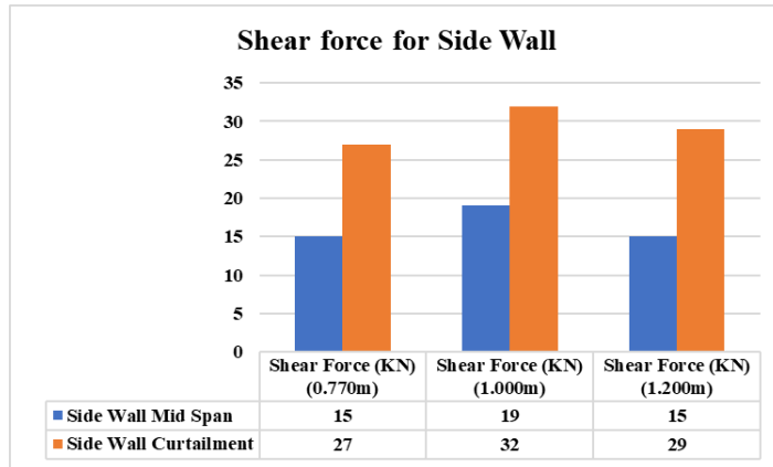
Graph No. 5 Shear force for Side Wall
