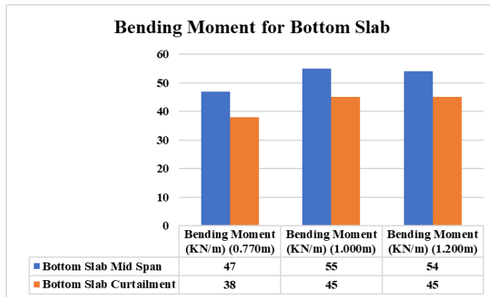
Graph No.3 Bending Moment for Bottom Slab
