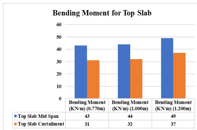
Graph No.1 Bending Moment for Top Slab
