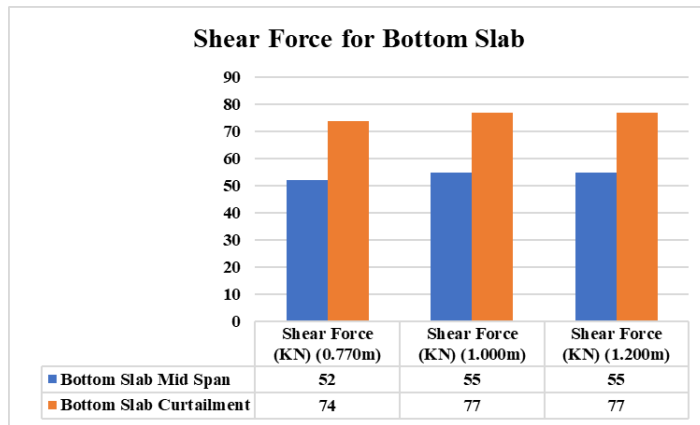
Graph No. 6 Shear force for Bottom Slab
