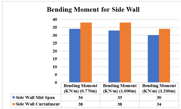
Graph No.2 Bending Moment for side wall
