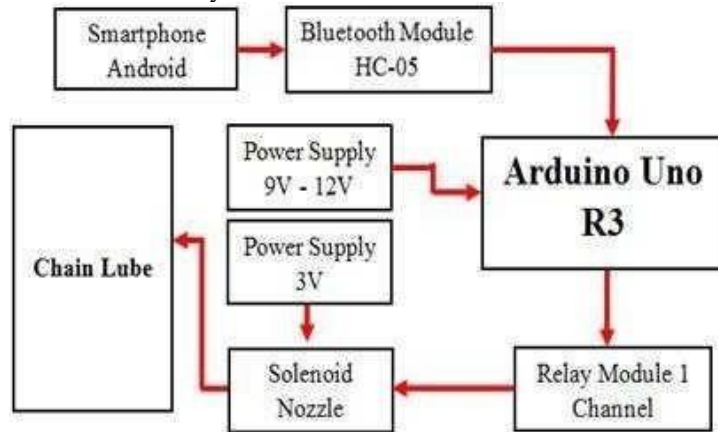
Fig.1 block diagram
