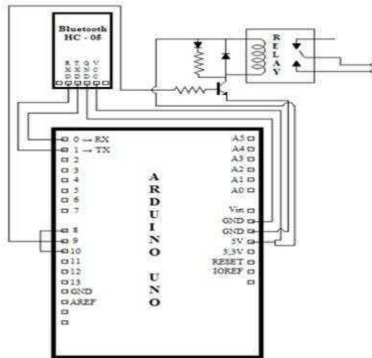
Fig. 3: Relay Module 1 Channel
