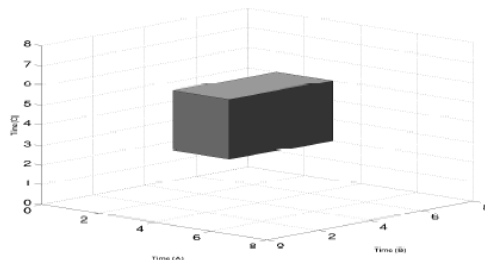
Figure-1: Hypercube Representation
