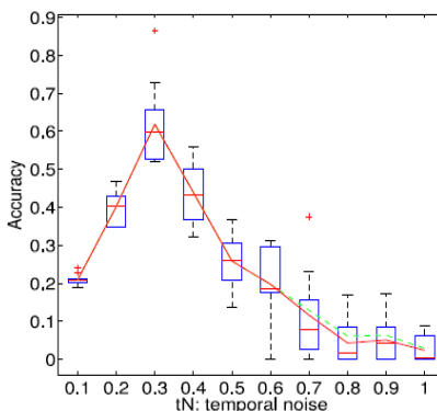
Figure-2: Accuracy vs Temporal Noise Graph
